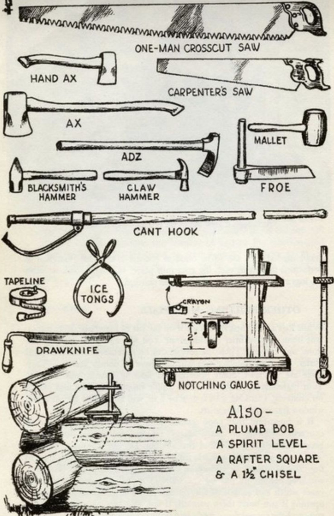
Fig. 6. Tools used for log cabin construction.
